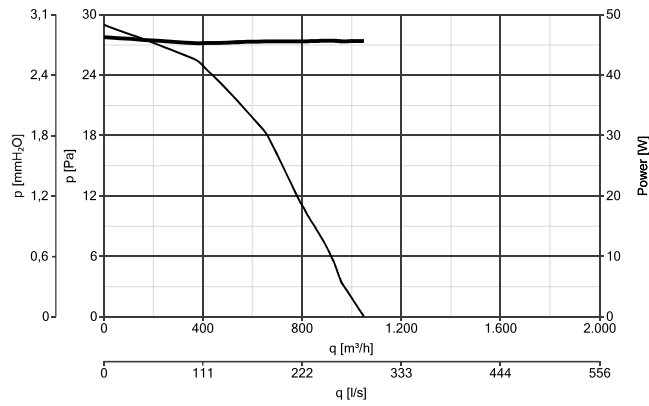
VORTICE 300/12" AR
