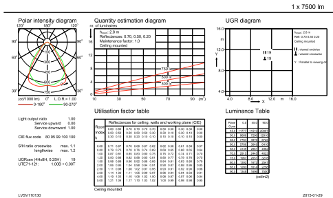
IFGU_4MX900 G3 581 1xLED75S/840 PSD MB-General uniform lighting
