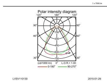
IFPC_4MX900 G3 581 1xLED75S/840 PSD MB-Polar Indoor (combined)
