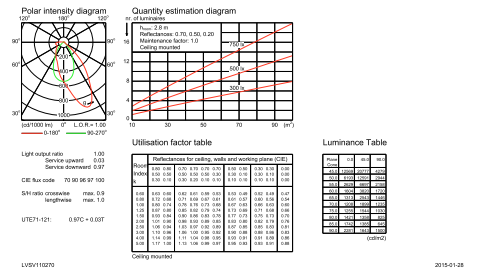
4MX900 G3 491 1xLED40S/840 PSU A30
