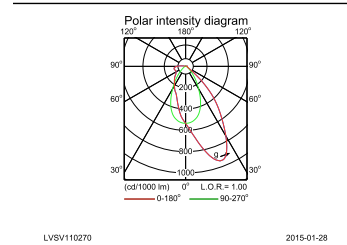
4MX900 G3 491 1xLED40S/840 PSU A30
