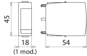
Dimension drawing DG MOD A NPE
