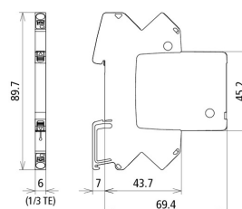
Dimension drawing BCO ML2 BD 48
