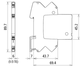
Dimension drawing BCO ML2 BE 12
