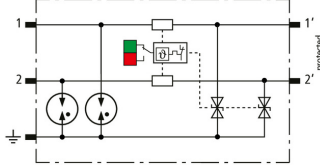
Basic circuit diagram BCO ML2 BE 12
