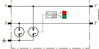
Basic circuit diagram BCO ML2 B 180
