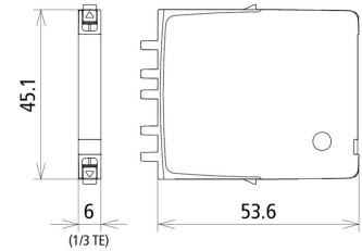
Dimension drawing BCO MOD ML2 BE 24
