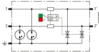
Basic circuit diagram BCO MOD ML2 BE 24
