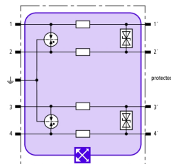
Basic circuit diagram BXT ML4 BD HF 5
