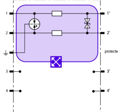
Basic circuit diagram BXT ML2 BD 180
