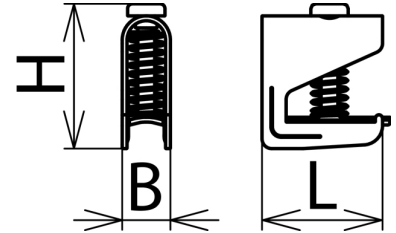
Dimension drawing SAK
