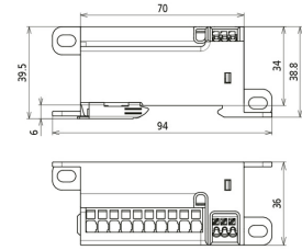
Dimension drawing DCOR 3P TT 275 FM
